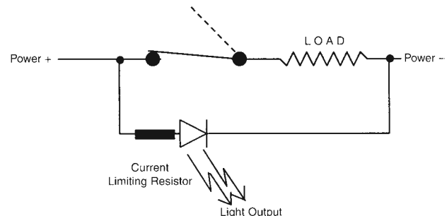
Figure 18. Wiring Diagram 3
