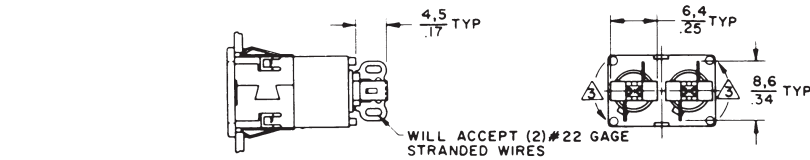
Solder Receptacle Installed (LED or Incandescent Lamp)
