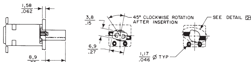
PWB Receptacle Installed (LED or Incandescent Lamp)
