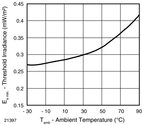
21397 E_{e, min.} - Threshold Irradiance ( \text{mW/m}^2 ) T_{amb} - Ambient Temperature ( ^{\circ}\text{C} ) Fig. 10 - Sensitivity vs. Ambient Temperature
