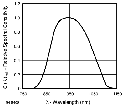
94 8408 S(\lambda)_{rel} - Relative Spectral Sensitivity \lambda - Wavelength (nm) Fig. 11 - Relative Spectral Sensitivity vs. Wavelength
