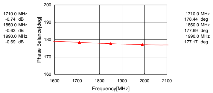
Phase Balance
