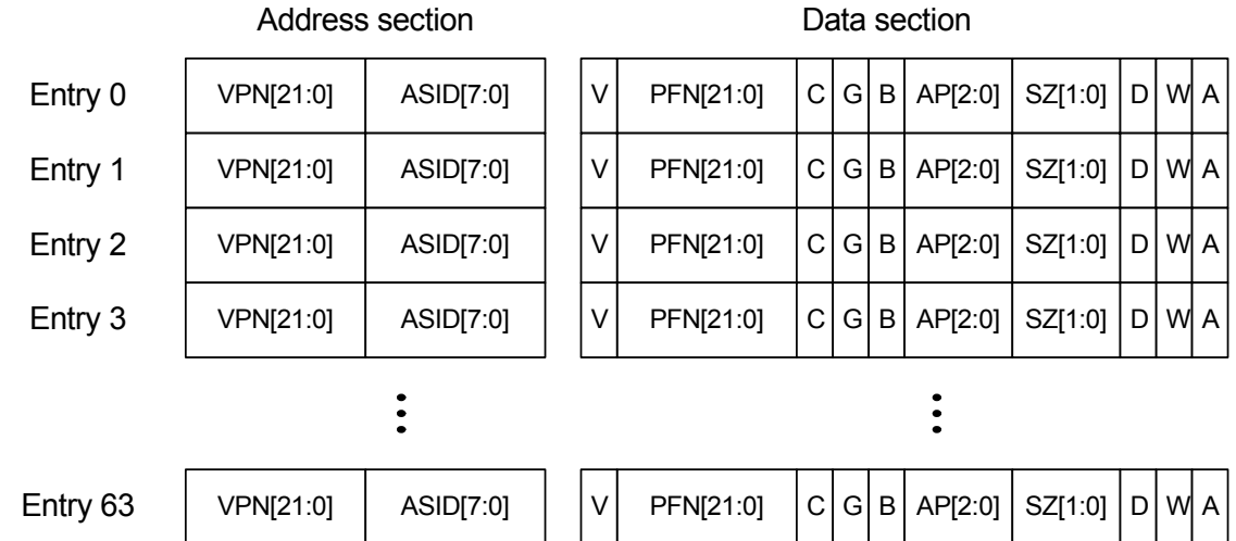
Figure 5-5. TLB organization
