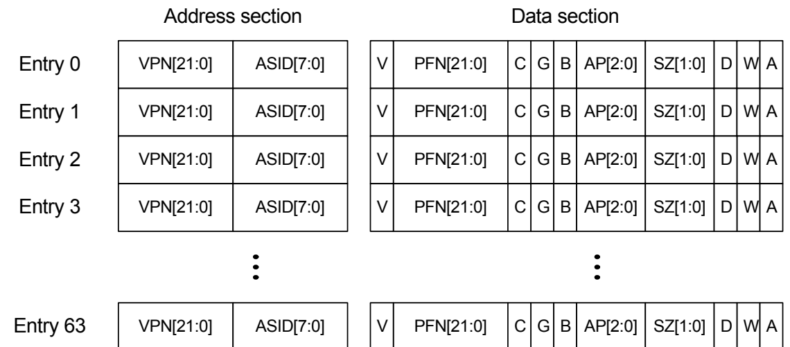
Figure 5-5. TLB organization
