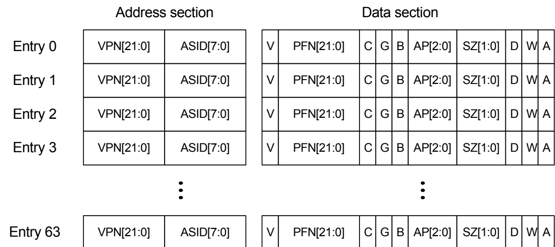
Figure 5-5. TLB organization
