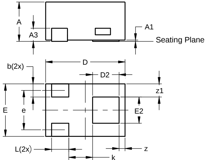
X2-DFN0604-3
