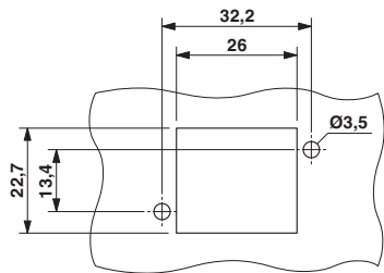
Panel cutout
