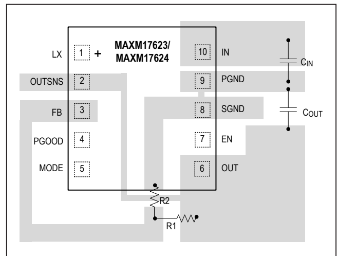
Figure 2. Layout Guidelines
