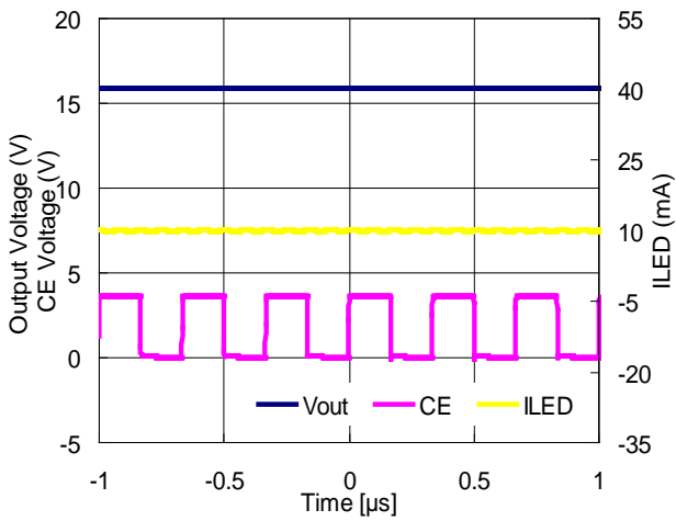
R1202N713D (CE Freq=300KHz)
