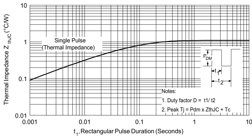
Fig. 4 - Maximum Thermal Impedance Z_{thJC} (Per Diode)
