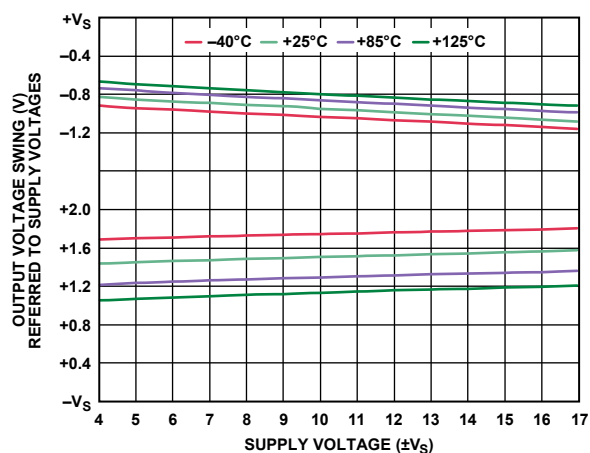
Figure 25. Output Voltage Swing vs. Supply Voltage, R_L = 2 k \Omega
