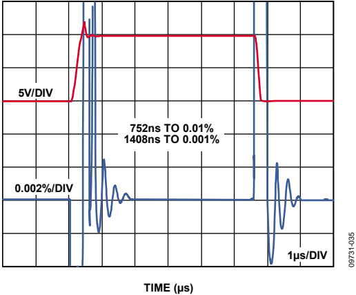
Figure 33. Large Signal Pulse Response and Settling Time, 10 V Step, V_S = \pm 15\text{ V}
