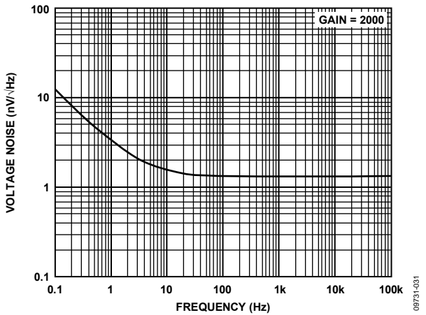
Figure 29. RTI Voltage Noise Spectral Density vs. Frequency
