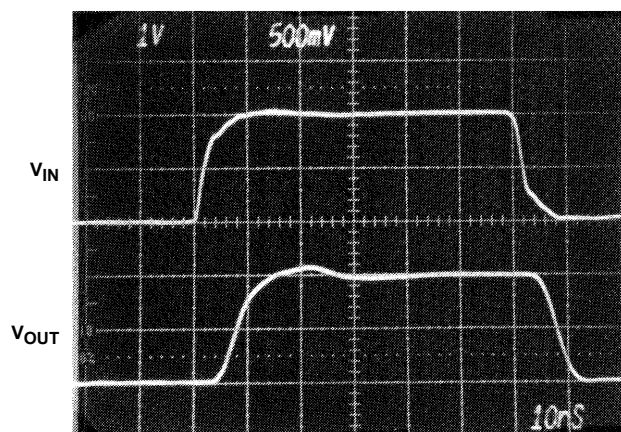
FIGURE 3. COAXIAL CABLE DRIVER - 50 \Omega SYSTEM
