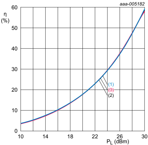
V_{SUP} = 3.6\text{ V} ; I_{CC(tot)} = 70\text{ mA} ; matched for ISM-915. (1) T_{amb} = -40^\circ\text{C} (2) T_{amb} = +25^\circ\text{C} (3) T_{amb} = +85^\circ\text{C}
