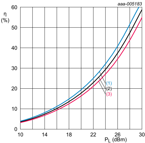
T_{amb} = 25^\circ\text{C} ; I_{CC(tot)} = 70\text{ mA} ; matched for ISM-915. (1) V_{SUP} = 3.3\text{ V} (2) V_{SUP} = 3.6\text{ V} (3) V_{SUP} = 3.9\text{ V}
