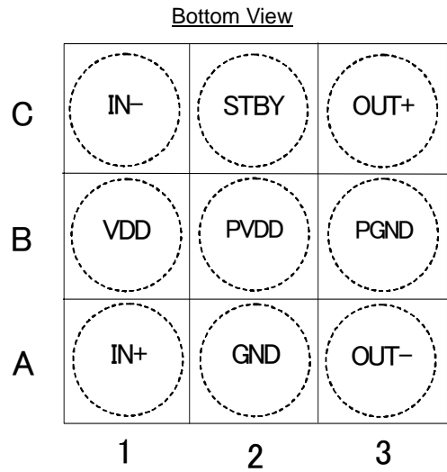
Figure.2 Pin configuration
