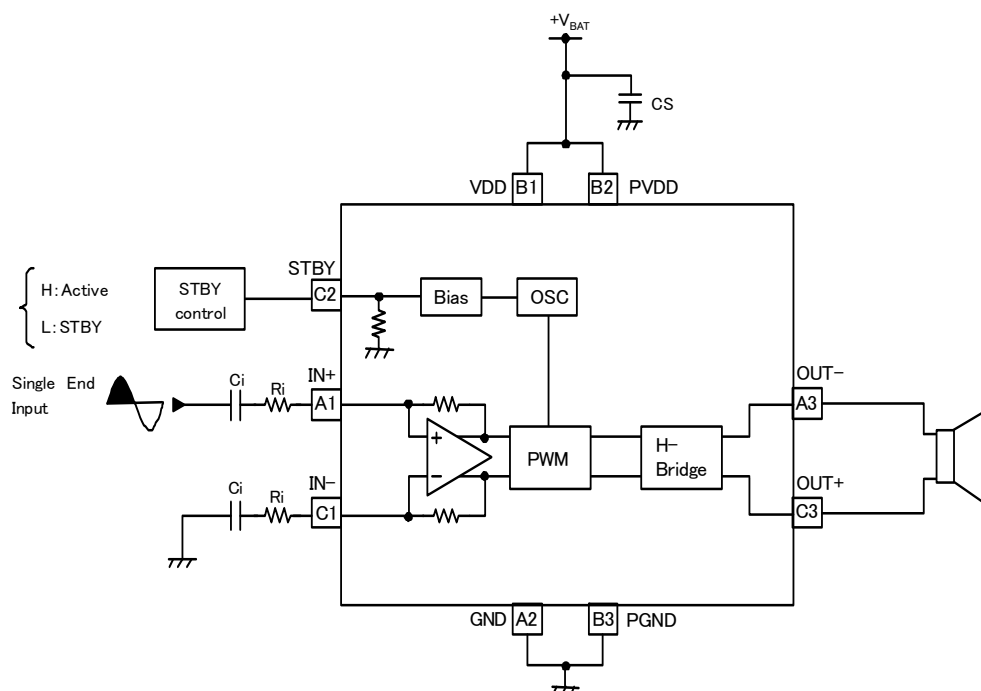
Figure.38 Single-Ended input
