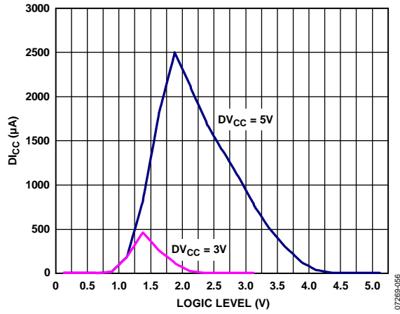
Figure 47. D CC vs. Logic Input Voltage
