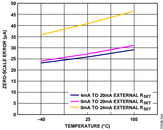
Figure 35. Zero-Scale Error vs. Temperature, External R SET Sense Resistor
