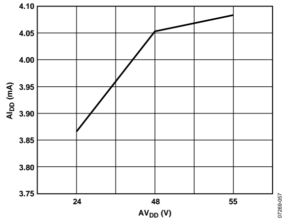
Figure 48. A LDD vs. A VDD , V OUT = 0 V
