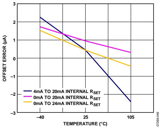
Figure 37. Offset Error vs. Temperature, Internal R SET Sense Resistor
