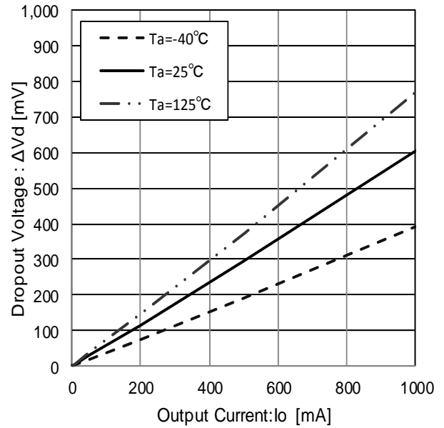
Figure 63. Dropout Voltage ( V_{cc} = V_o \times 0.95\text{V} )
