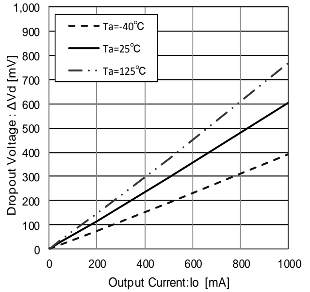
Figure 51. Dropout Voltage (Vcc=Vo×0.95V)
