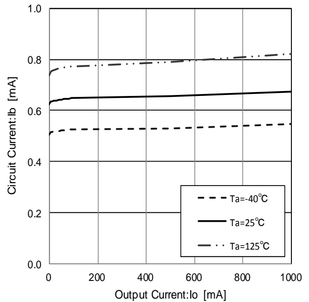
Figure 30. Circuit Current
