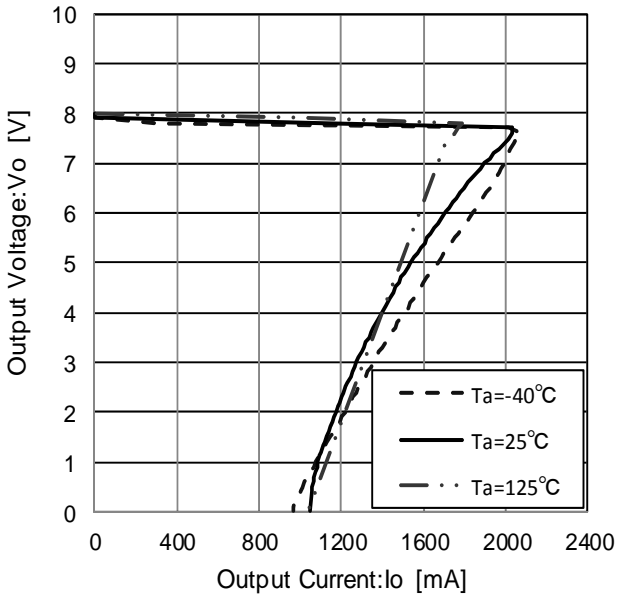
Figure 50. Load Regulation
