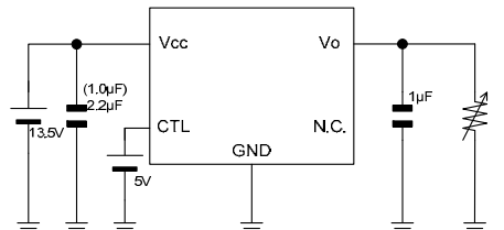
Measurement setup for Figure 30, 42, 54 and 66
