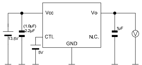
Measurement setup for Figure 33, 45, 57 and 69
