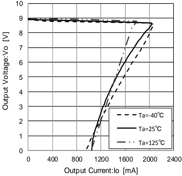
Figure 62. Load Regulation
