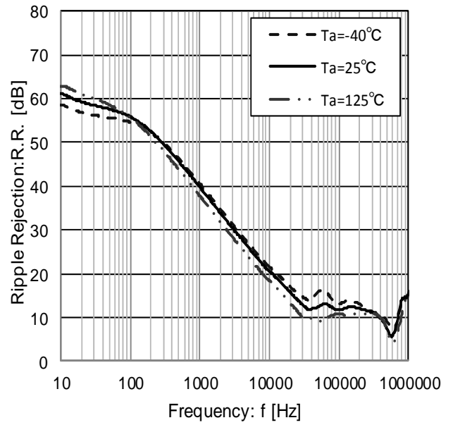
Figure 28. Ripple Rejection (Ilo=100mA)
