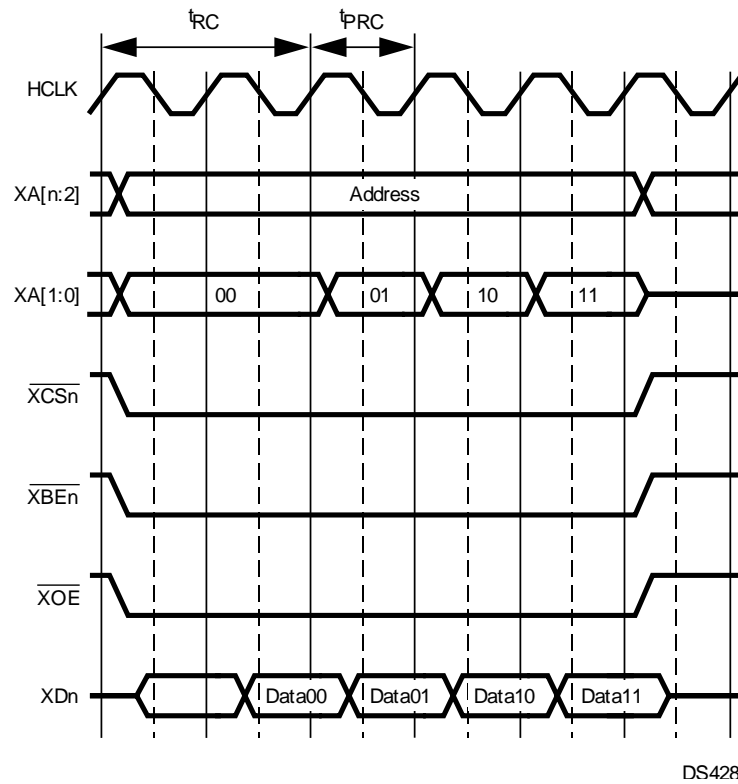
Figure 10-3. Page-Mode Read Cycle Timing
