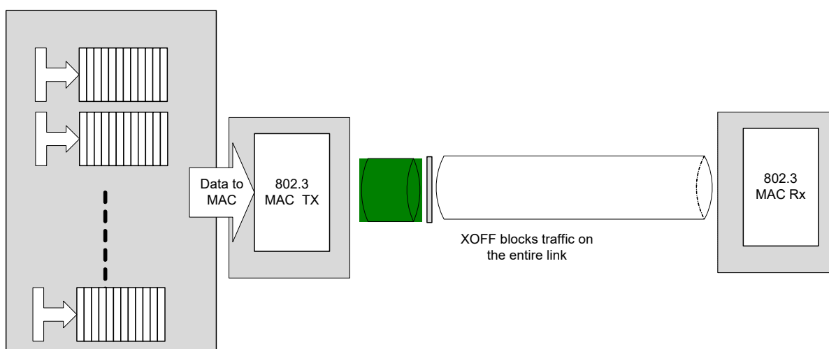
Figure 3-9. 802.3X Link Flow Control (PAUSE)
