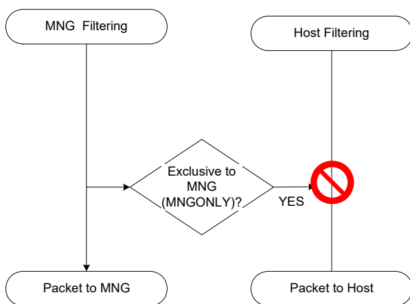
Figure 7-4. Manageability/Host Filtering
