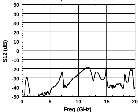
NJG1106KB2 S12 vs. Freq(to 20GHz)
