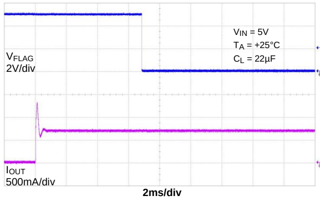
3 \Omega Load Connected to Enabled Device
