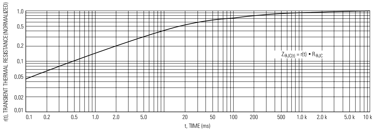
Figure 8. Thermal Response
