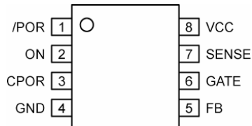
8-Pin SOIC (M)
