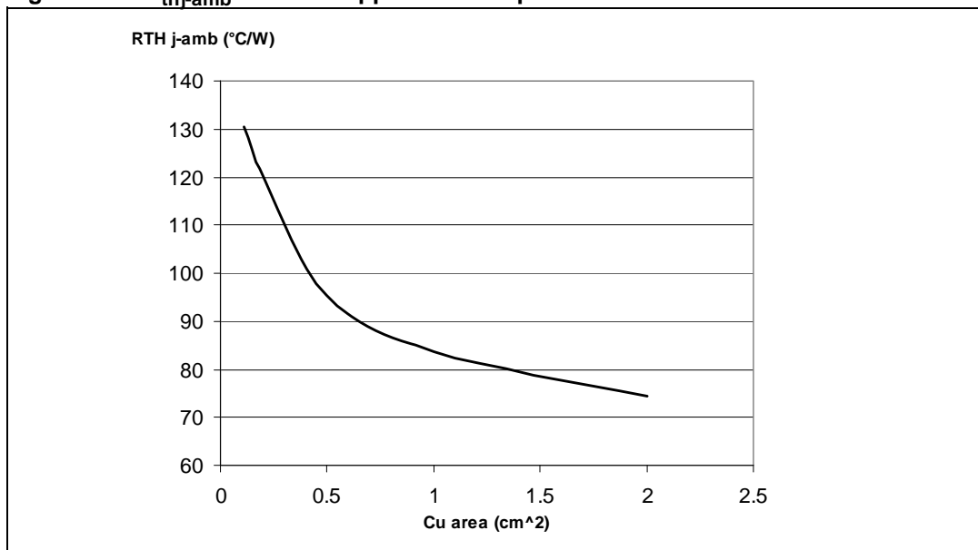
Figure 39. R_{thj-amb} vs PCB copper area in open box free air condition
