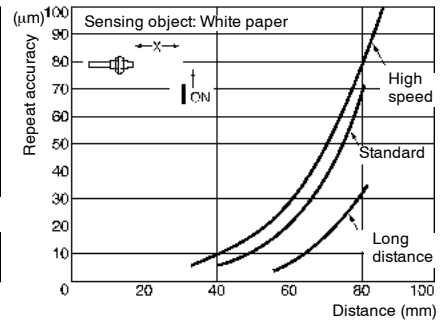
Repeat Accuracy vs. Sensing Distance E32-DC200 with E3X-DAN amplifier (Reflective)
