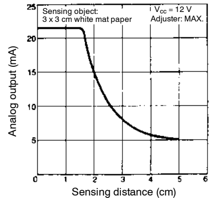
E32-DC200D/D4 with E3XA-CC4A analog amplifier
