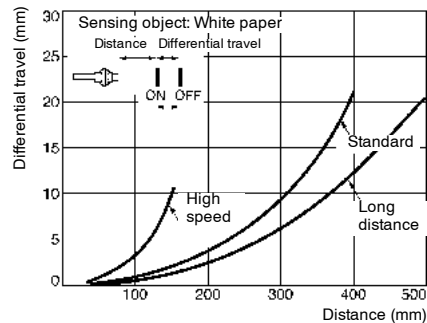
Differential Travel vs. Sensing Distance E32-D11L with E3X-DAN amplifier (Reflective)
