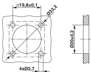
M12 flush-type plug, square flange
