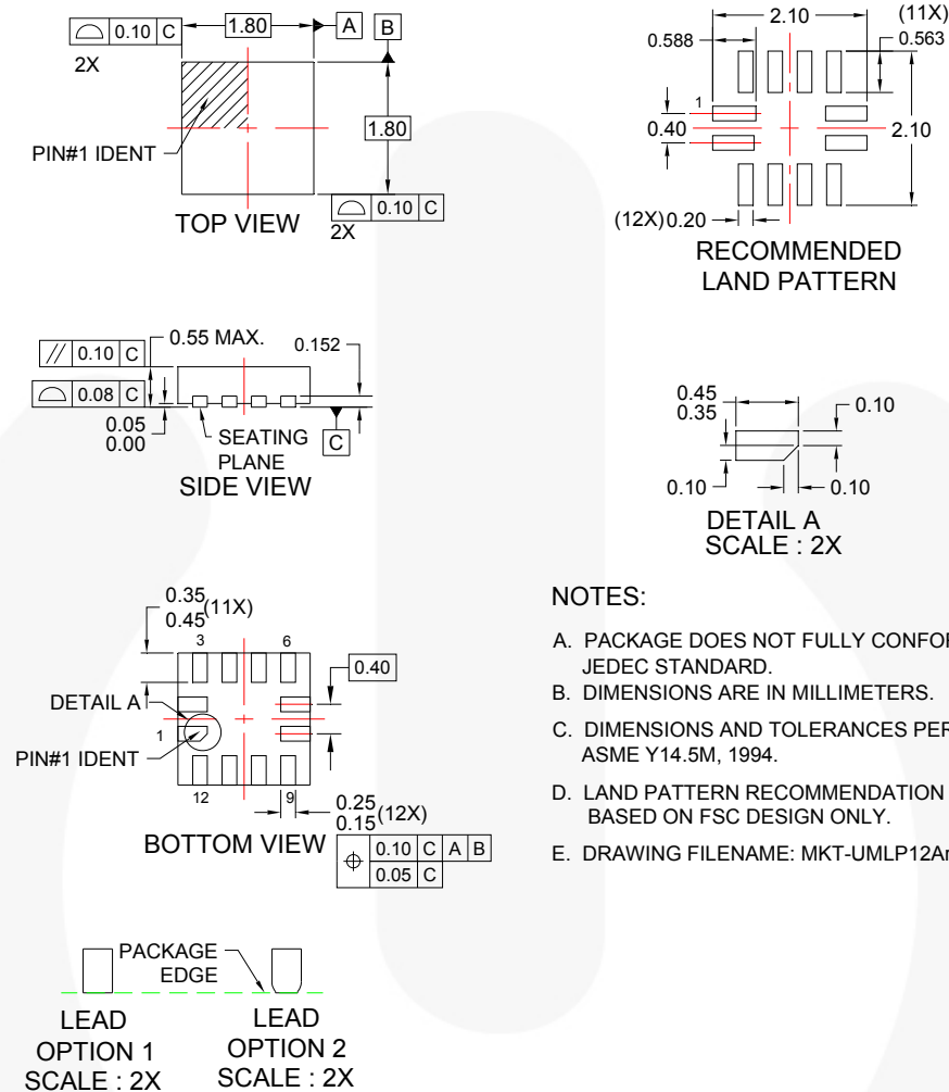
Figure 15. 12-Lead, Ultrathin Molded Leadless Package (UMLP)
