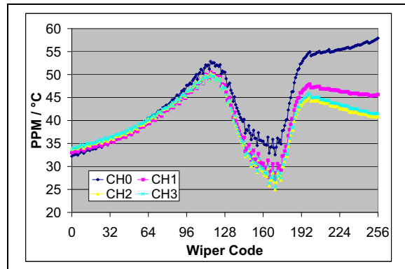
FIGURE 2-40: 10\text{ k}\Omega – R_{WB} PPM/°C vs. Wiper Setting. (R_{BW(\text{code}=n, 125^\circ\text{C})} - R_{BW(\text{code}=n, -40^\circ\text{C})}) / R_{BW(\text{code}=256, 25^\circ\text{C})} / 165^\circ\text{C} * 1,000,000 ( V_{DD} = 3.0\text{V} , I_W = 150\ \mu\text{A} ).
