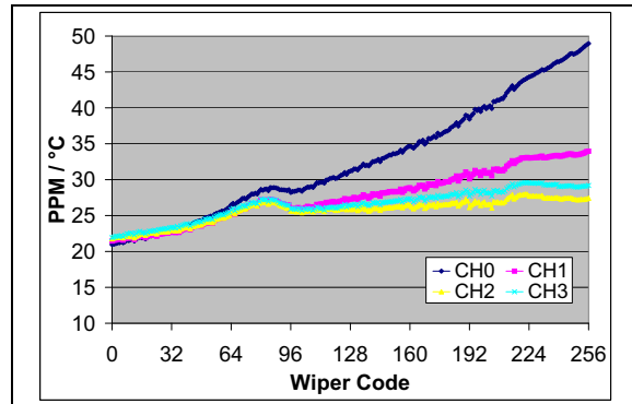
FIGURE 2-39: 10\text{ k}\Omega – R_{WB} PPM/°C vs. Wiper Setting. (R_{BW(\text{code}=n, 125^\circ\text{C})} - R_{BW(\text{code}=n, -40^\circ\text{C})}) / R_{BW(\text{code}=256, 25^\circ\text{C})} / 165^\circ\text{C} * 1,000,000 ( V_{DD} = 5.5\text{V} , I_W = 150\ \mu\text{A} ).
