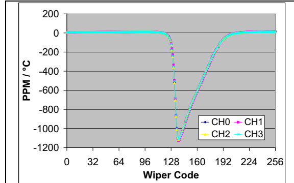
FIGURE 2-80: 100 k \Omega – R_{WB} PPM/ ^\circ\text{C} vs. Wiper Setting. ( R_{BW}(\text{code}=n, 125^\circ\text{C}) - R_{BW}(\text{code}=n, -40^\circ\text{C}) ) / R_{BW}(\text{code} = 256, 25^\circ\text{C}) / 165^\circ\text{C} * 1,000,000 ) ( V_{DD} = 3.0\text{V} , I_W = 24\text{ }\mu\text{A} ).
