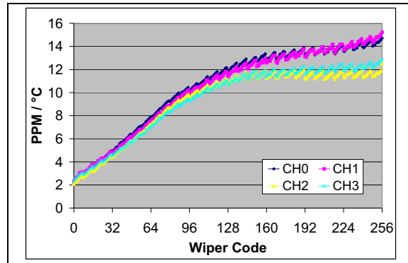
FIGURE 2-79: 100 k \Omega – R_{WB} PPM/ ^\circ\text{C} vs. Wiper Setting. ( R_{BW}(\text{code}=n, 125^\circ\text{C}) - R_{BW}(\text{code}=n, -40^\circ\text{C}) ) / R_{BW}(\text{code} = 256, 25^\circ\text{C}) / 165^\circ\text{C} * 1,000,000 ) ( V_{DD} = 5.5\text{V} , I_W = 45\text{ }\mu\text{A} ).
