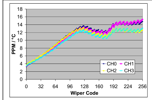
FIGURE 2-80: 100 k \Omega – R_{WB} PPM/ ^\circ\text{C} vs. Wiper Setting. ( R_{BW}(\text{code}=n, 125^\circ\text{C}) - R_{BW}(\text{code}=n, -40^\circ\text{C}) ) / R_{BW}(\text{code} = 256, 25^\circ\text{C}) / 165^\circ\text{C} * 1,000,000 ) ( V_{DD} = 3.0\text{V} , I_W = 24\text{ }\mu\text{A} ).
