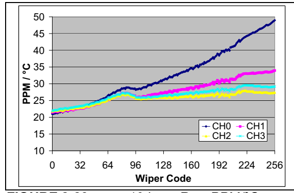
FIGURE 2-39: 10 kΩ – R_{WB} PPM/°C vs. Wiper Setting. (R_{BW}(\text{code}=n, 125^\circ\text{C}) - R_{BW}(\text{code}=n, -40^\circ\text{C})) / R_{BW}(\text{code} = 256, 25^\circ\text{C}) / 165^\circ\text{C} * 1,000,000 ( V_{DD} = 5.5\text{V} , I_W = 150\ \mu\text{A} ).
