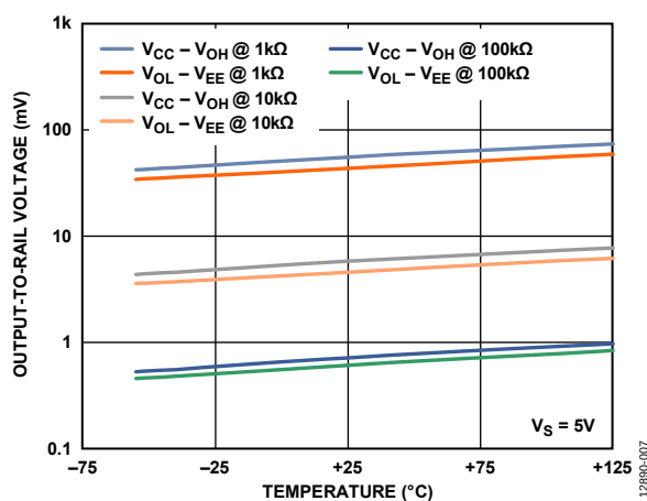
Figure 7. Output-to-Rail Voltage vs. Temperature (5 V)
