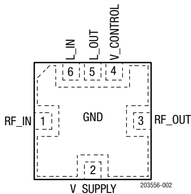
Figure 2. SKY12239-11 Pinout (Top View)
