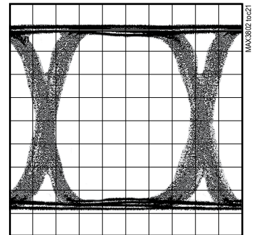
60ps/div (2.5Gbps)
