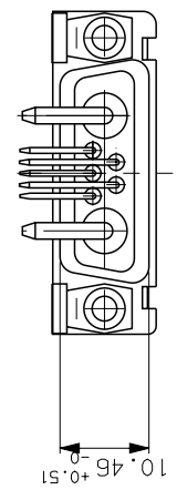
LAYOUT DIMENSIONS (after plating) CONNECTOR SIDE VIEW
