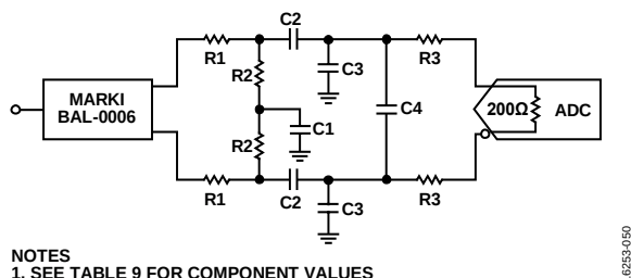
Figure 45. Differential Transformer-Coupled Configuration for the AD9697
