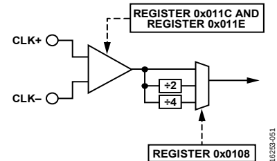
Figure 56. Clock Divider Circuit
