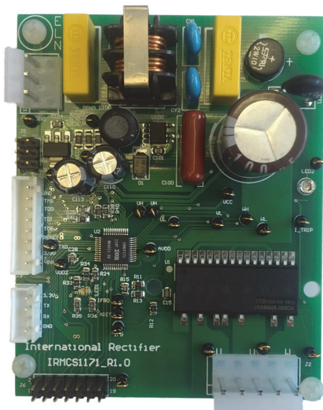
Figure 4: Reference design board featuring the \mu IPM™-DIP module and the iMotion™ IRMCF171 digital control IC
