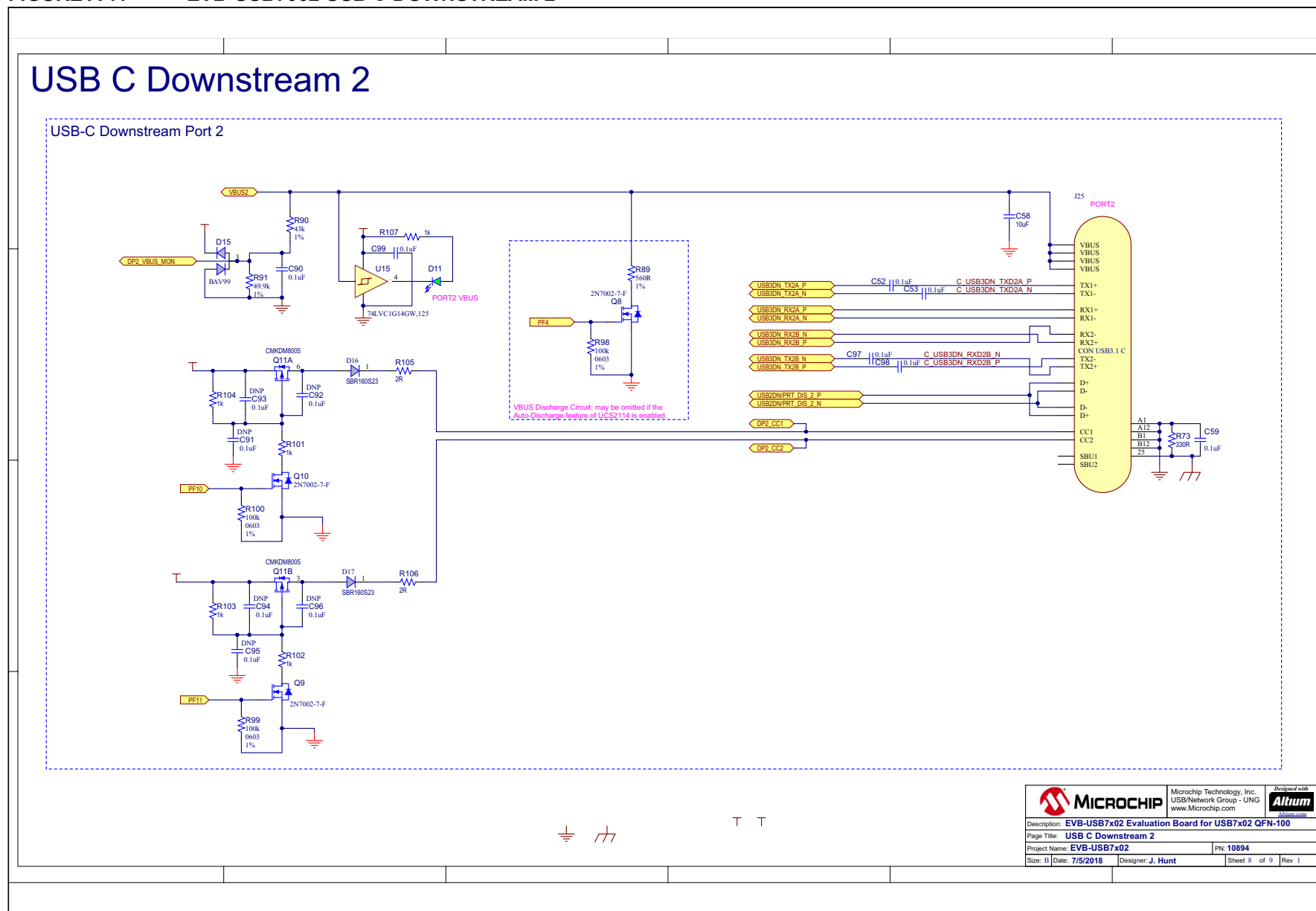
FIGURE A-7: EVB-USB7002 USB C DOWNSTREAM 2
