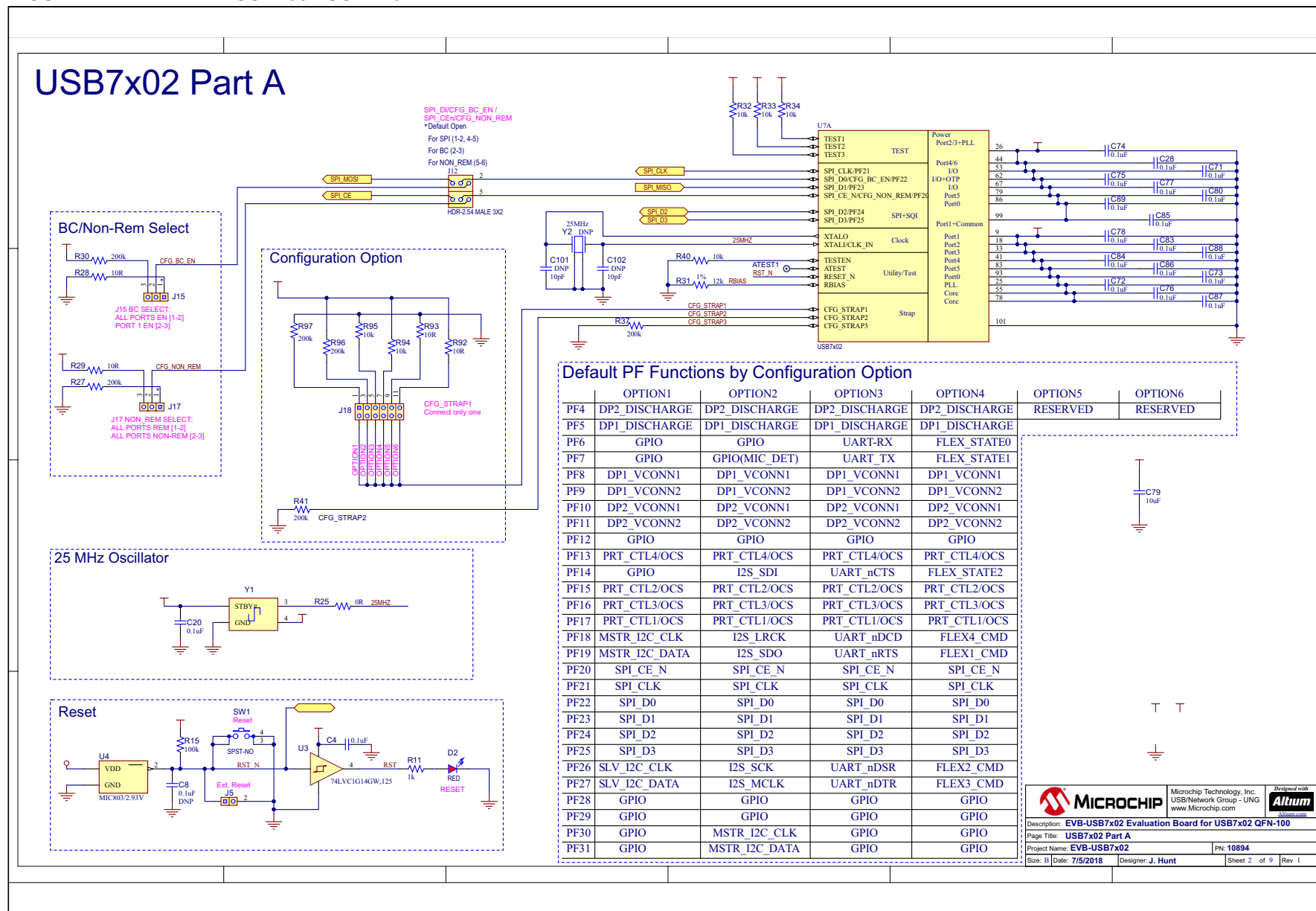
FIGURE A-1: EVB-USB7002 USB7X02 PART A
