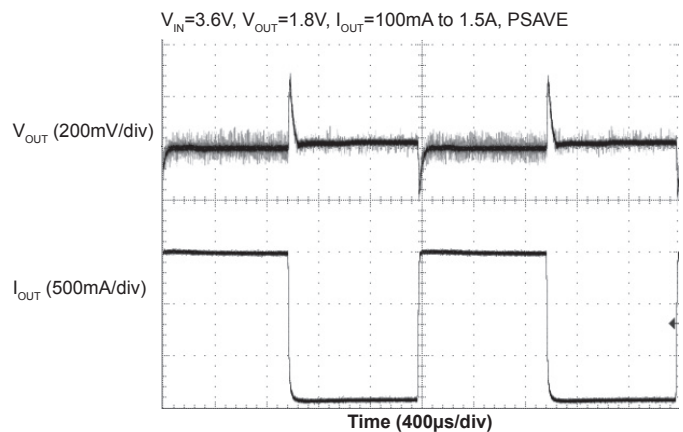
Load Transient Response-4
