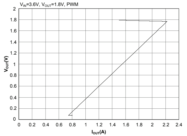
Current Limit
