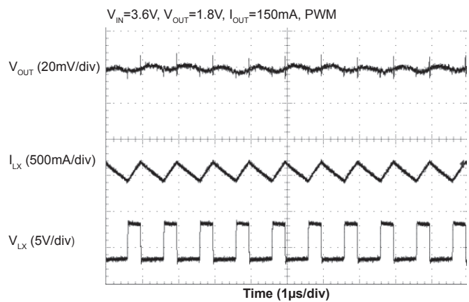
PWM Operation
