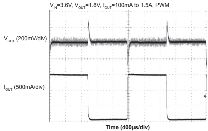
Load Transient Response-2
