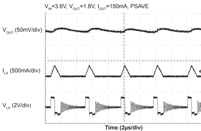
PSAVE Operation
