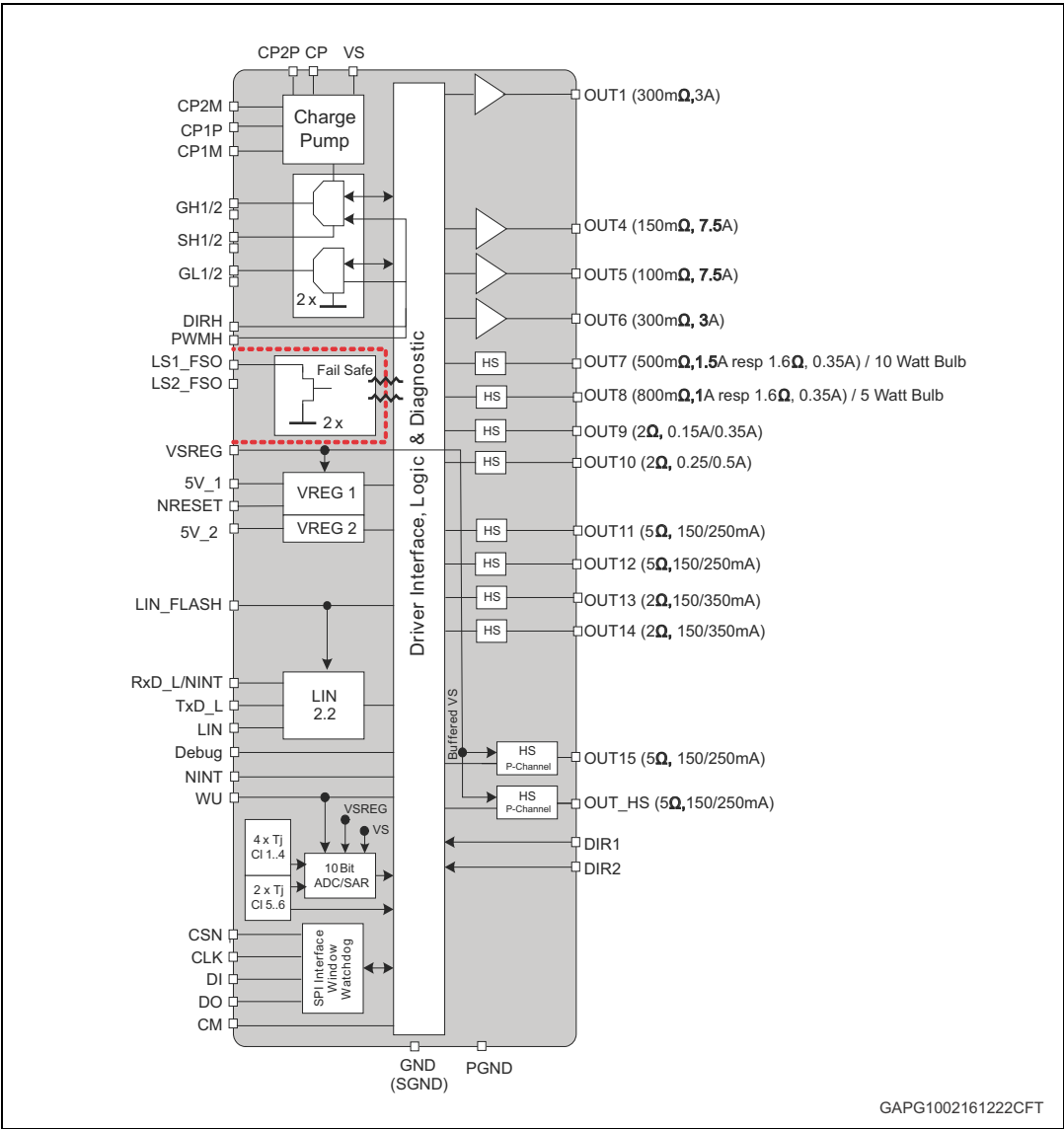
Figure 1. Block diagram
