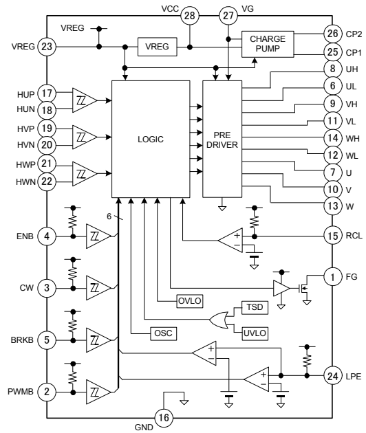
Figure 3. Block diagram
