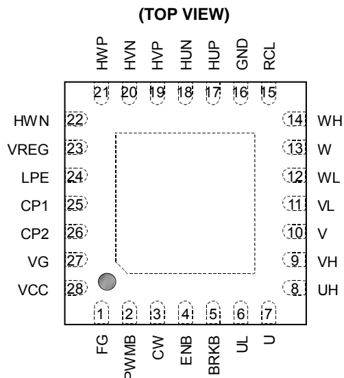
Figure 2. Pin configuration
