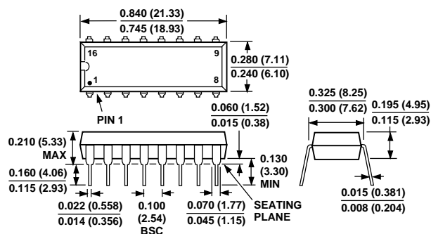
Plastic DIP (N-16)
